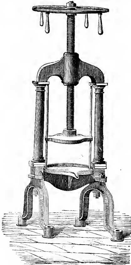
EXTRACTION PRESS.
